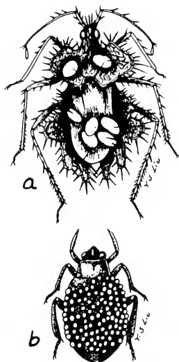
Fig. 16. Eggs on the back of male insects: a, Phylonomorpha laciniata ; b, Western water bug, Abedus sp.
